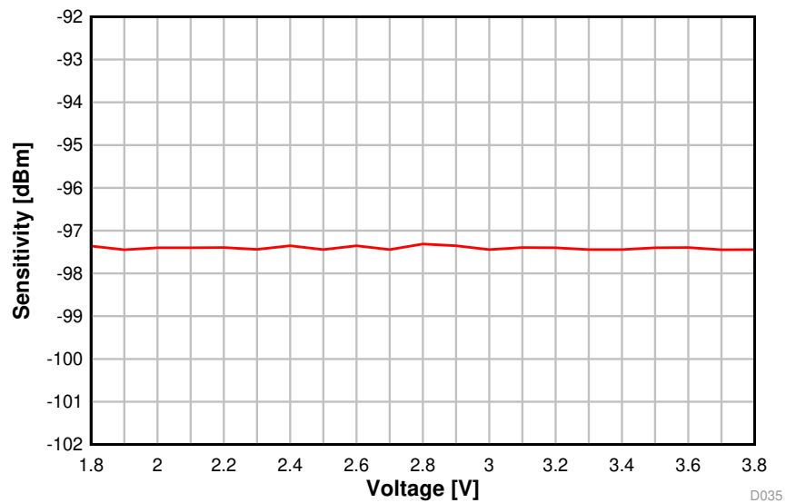
Figure 5-14. Sensitivity vs. Supply Voltage (VDD5) (BLE 1 Mbps, 2.44 GHz, DCDC Off)
