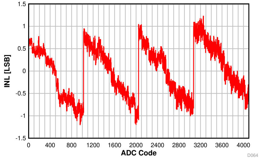
Figure 5-23. INL vs. ADC Code
