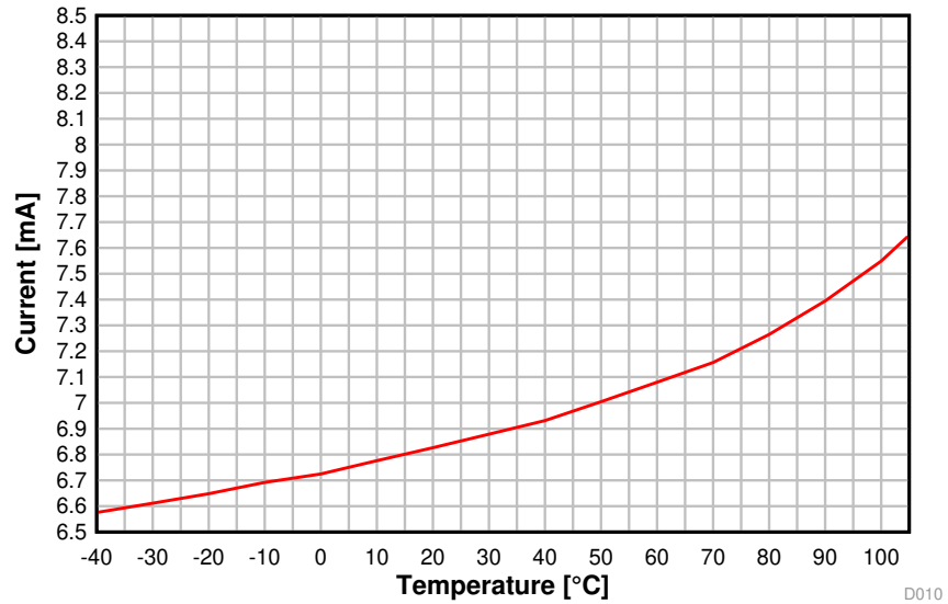
RX Current vs. Temperature BLE 1 Mbps, 2.44 GHz
