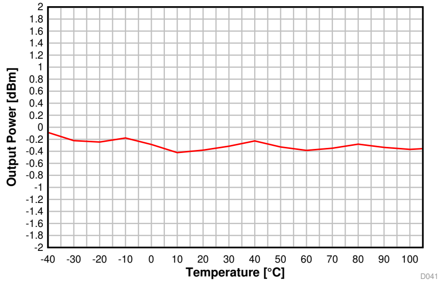
Figure 5-15. Output Power vs. Temperature (BLE 1 Mbps, 2.44 GHz)
