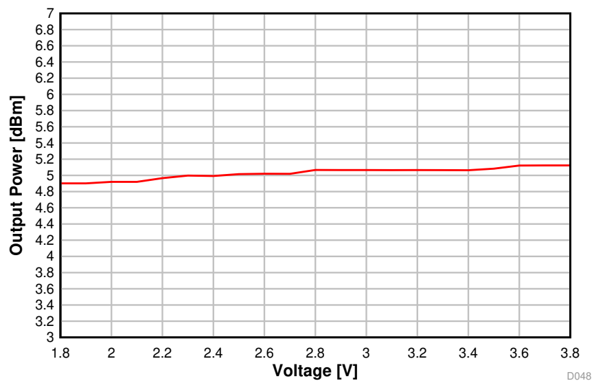
Figure 5-18. Output Power vs. Supply Voltage (VDDS) (BLE 1 Mbps, 2.44 GHz, +5 dBm)
