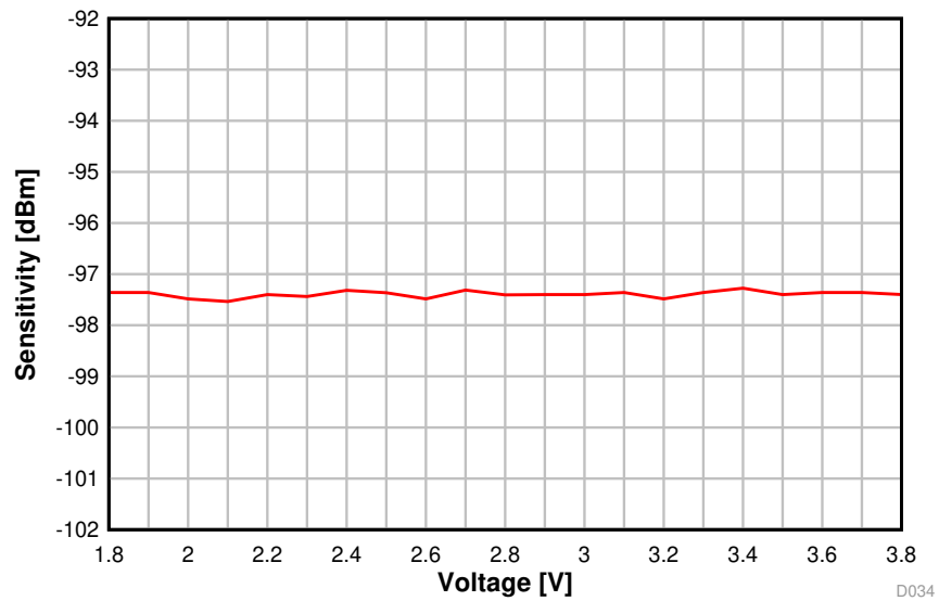
Figure 5-13. Sensitivity vs. Supply Voltage (VDD5) (BLE 1 Mbps, 2.44 GHz)
