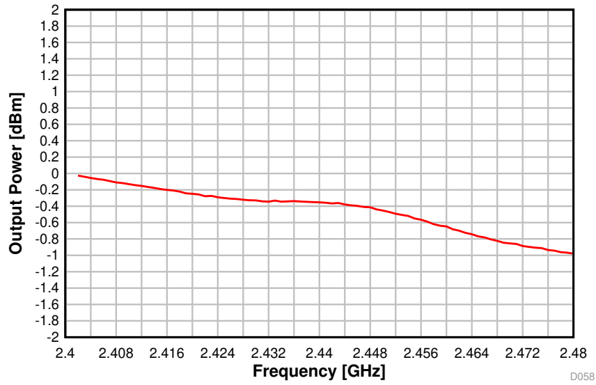
Figure 5-19. Output Power vs. Frequency (BLE 1 Mbps, 2.44 GHz)
