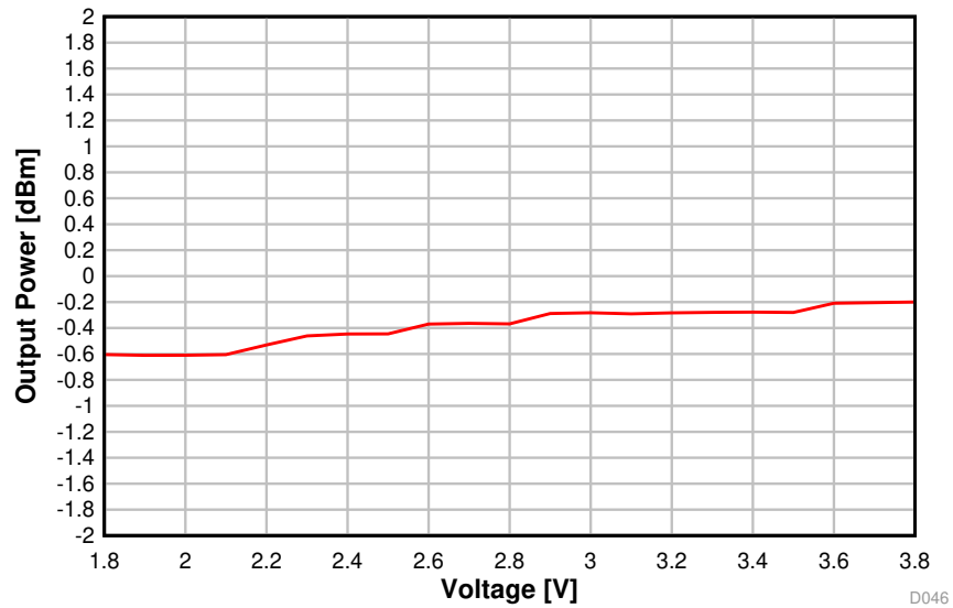
Figure 5-17. Output Power vs. Supply Voltage (VDDS) (BLE 1 Mbps, 2.44 GHz)
