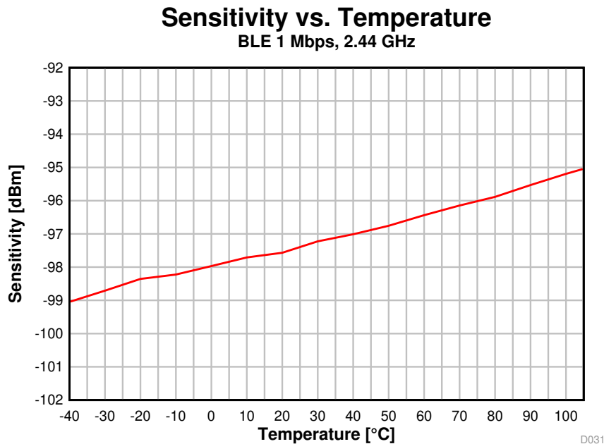
Figure 5-12. Sensitivity vs. Temperature (BLE 1 Mbps, 2.44 GHz)
