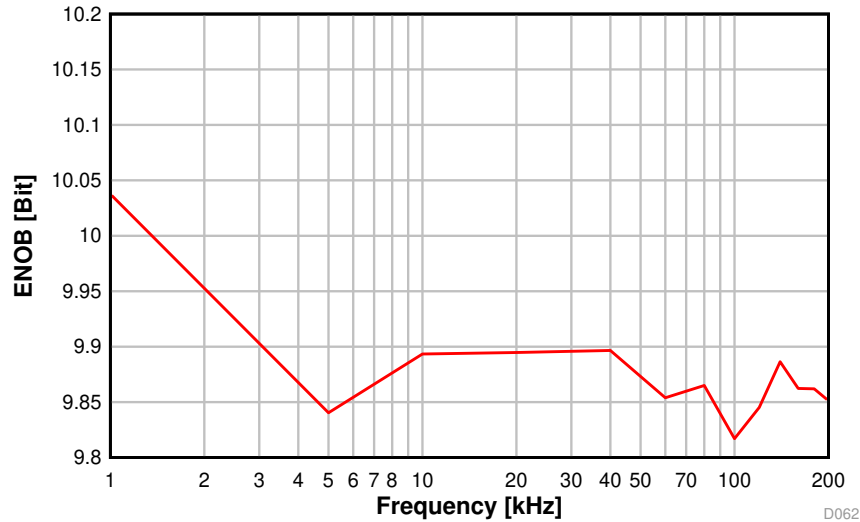
ENOB vs. Sampling Frequency V_{in} = 3.0\text{ V} Sine wave, Internal reference, F_{in} = F_s / 10
