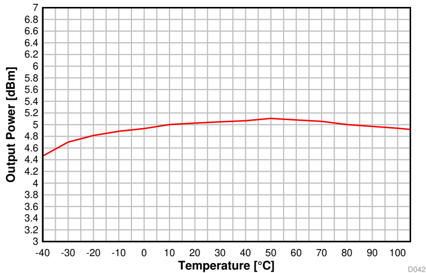
Figure 5-16. Output Power vs. Temperature (BLE 1 Mbps, 2.44 GHz, +5 dBm)
