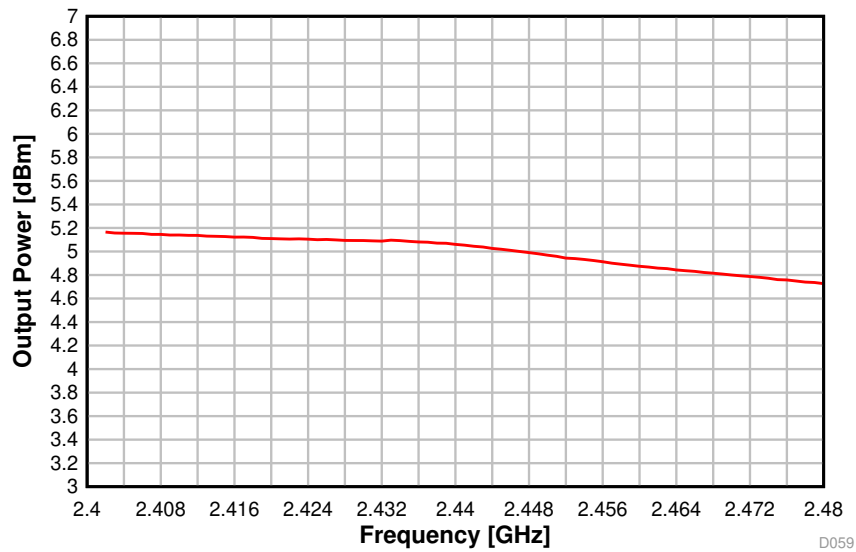
Figure 5-20. Output Power vs. Frequency (BLE 1 Mbps, 2.44 GHz, +5 dBm)
