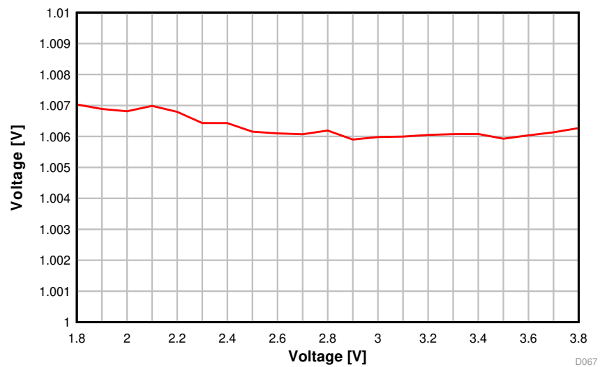
Figure 5-26. ADC Accuracy vs. Supply Voltage (VDD5)
