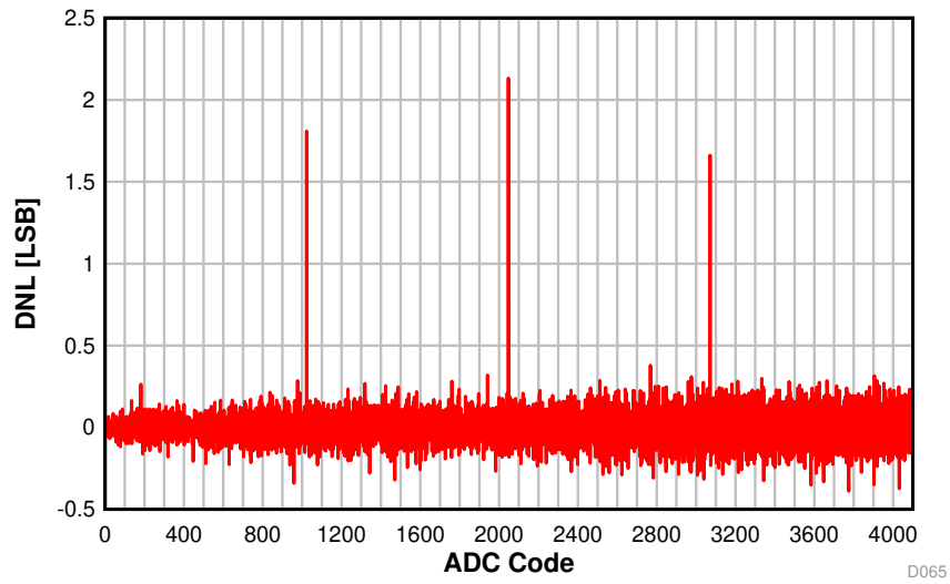
Figure 5-24. DNL vs. ADC Code
